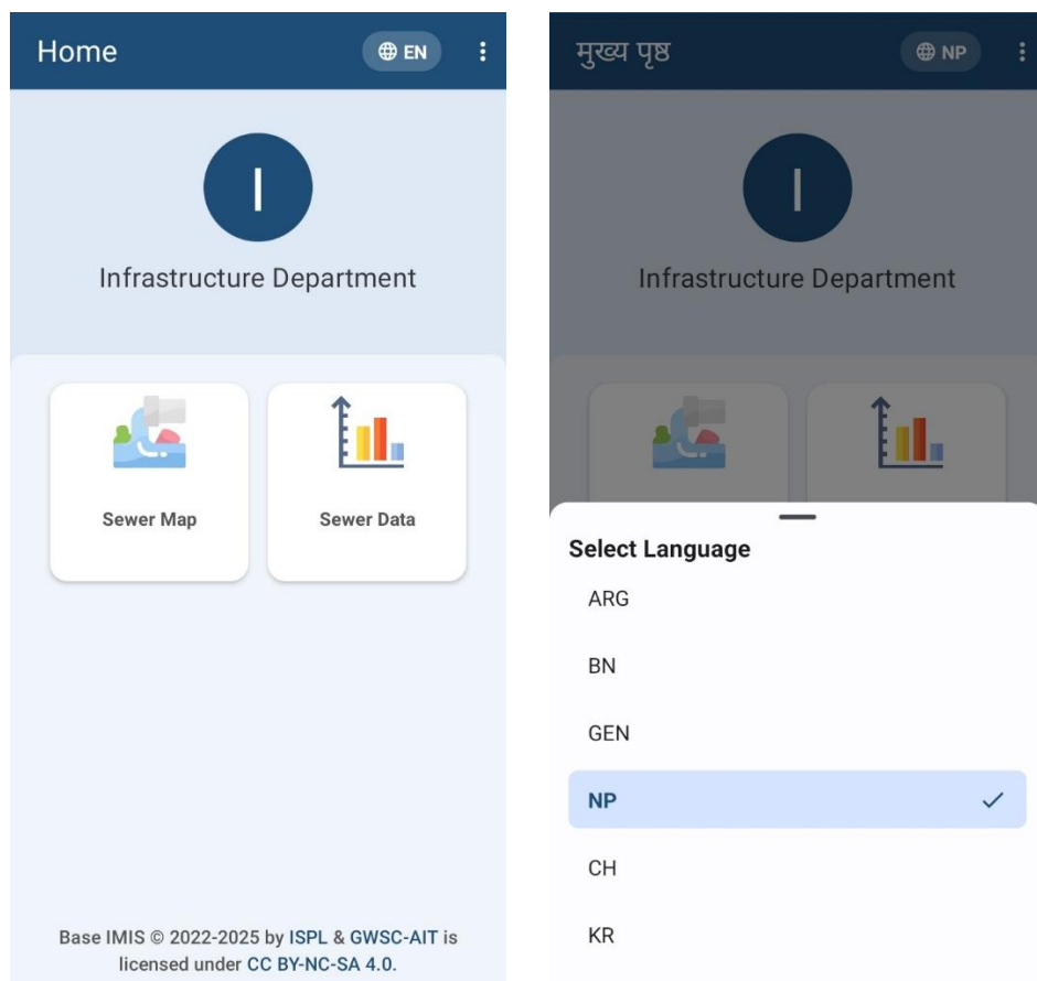
Figure 3-1 Dashboard
