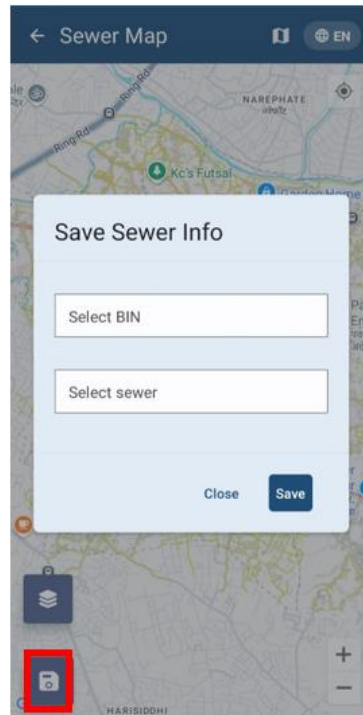
Figure 4-5 Sewer Form
