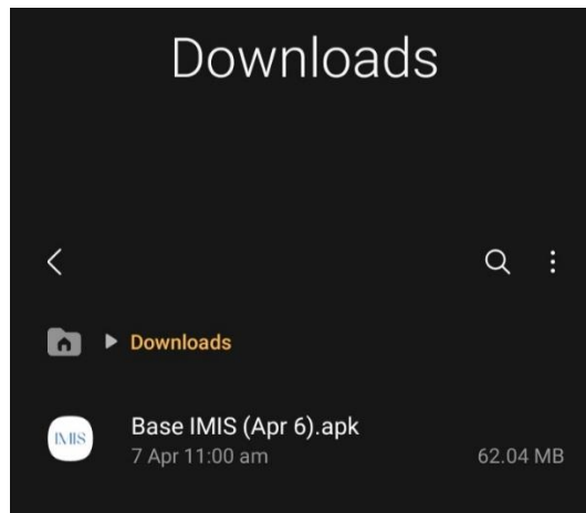
Figure 1-1 APK file
