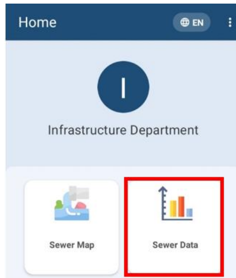
Figure 5-1 Sewer Data
