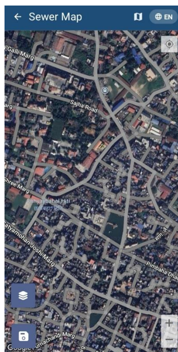
Figure 4-2 Map Interface
