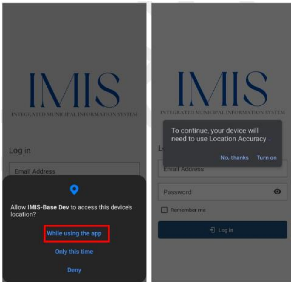
Figure 6-1 Location Permission
